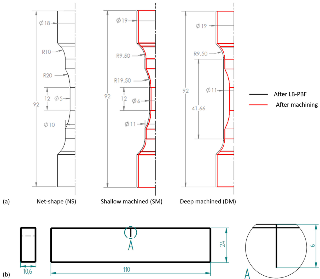
Fig. 3. Drawing of specimens: (a) uniaxial fatigue according to ASTM E466 [39], geometries before machining (in black) and after machining (in red); (b) single-edge bending (SE(B)) FCG after machining according to BS ISO 12108 [40]. (For interpretation of the references to colour in this figure legend, the reader is referred to the web version of this article.)
