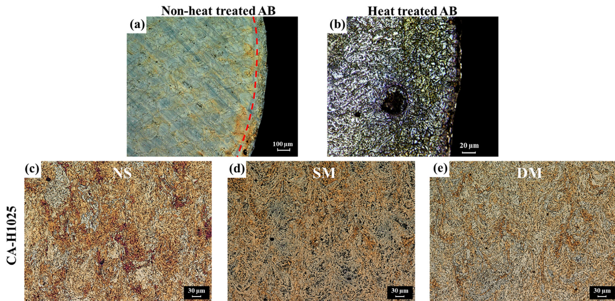
Fig. 4. Overview of microstructures before and after CA-H1025 heat treatment.
