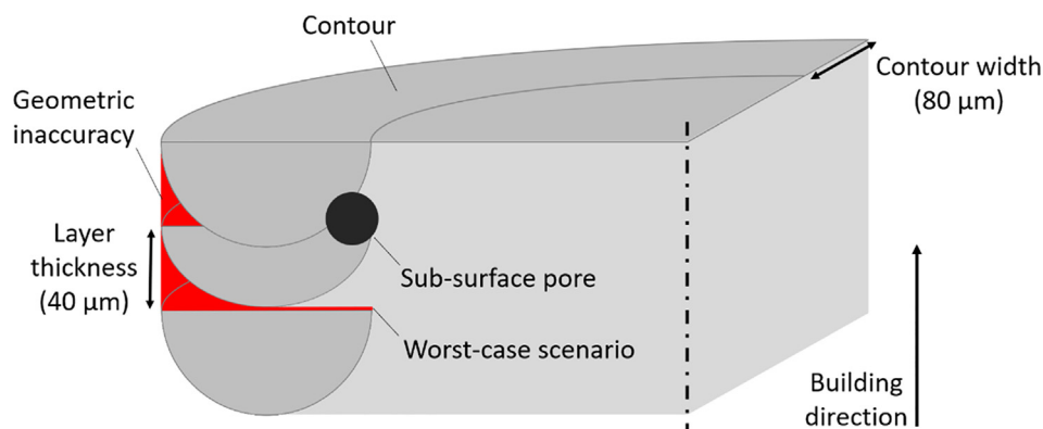
Fig. 14. Simplified schematic of geometric inaccuracy and sub-surface porosity created by contouring strategy.
