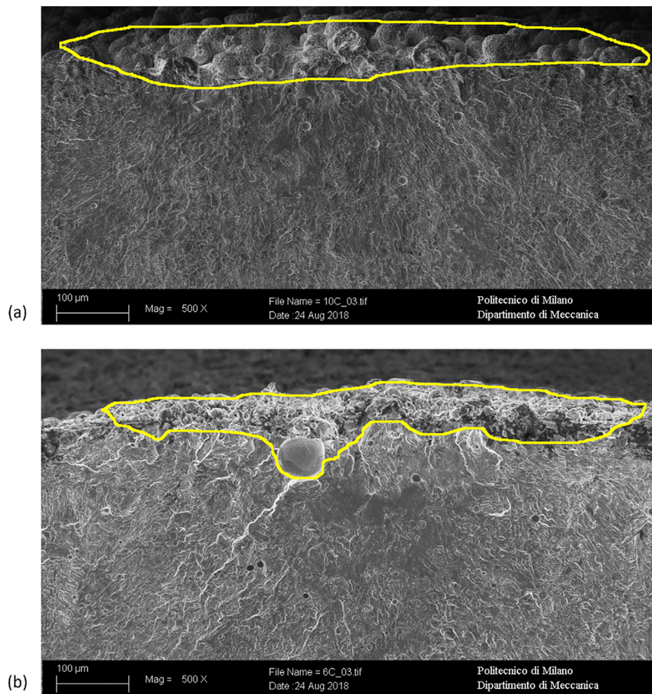
Fig. 10. Examples of typical fracture surfaces for the NS condition: (a) a specimen fractured after 6.22 \times 10^5 cycles subjected to a stress amplitude of 250 MPa; and (b) a specimen fractured after 7.42 \times 10^5 cycles subjected to a stress amplitude of 300 MPa showing a sub-surface pore with 65 \mu\text{m} diameter.
