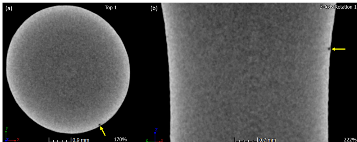
Fig. 5. Example of sub-surface, and close-to-surface pores detected via X-ray micro-CT. The arrows show its position in (a) radial and (b) longitudinal directions.
