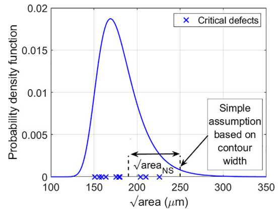
Fig. 15. LEVD of experimental surface feature size for NS condition compared to the conservative estimate obtained via Eq. (5).
