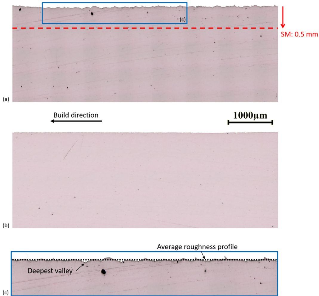
Fig. 6. Examples of polished sections for: (a) NS; and (b) SM specimens (similar results were obtained for DM specimens); (c) detail of roughness profile for NS condition.
