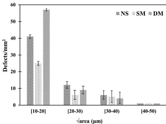
Fig. 7. Porosity size distribution obtained from polished sections.
