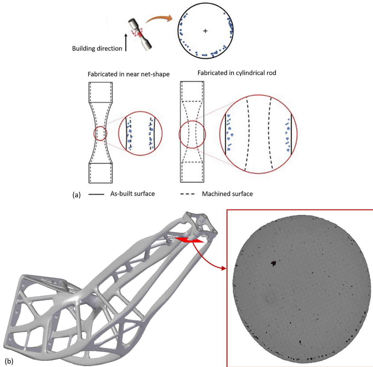
Fig. 1. Typical sub-surface features in net-shape parts: (a) sub-surface porosity generated by the LB-PBF process in net-shape or machined specimens (adapted from [1]); (b) sub-surface porosity in the down-skin region of an inclined AlSi10Mg part produced without supports (adapted from [7]).
