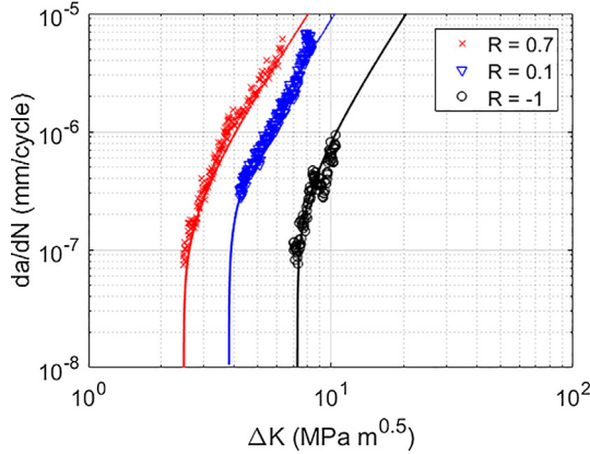
Fig. 8. NASGRO fit to the experimental FCG data obtained via NASGRO software.
