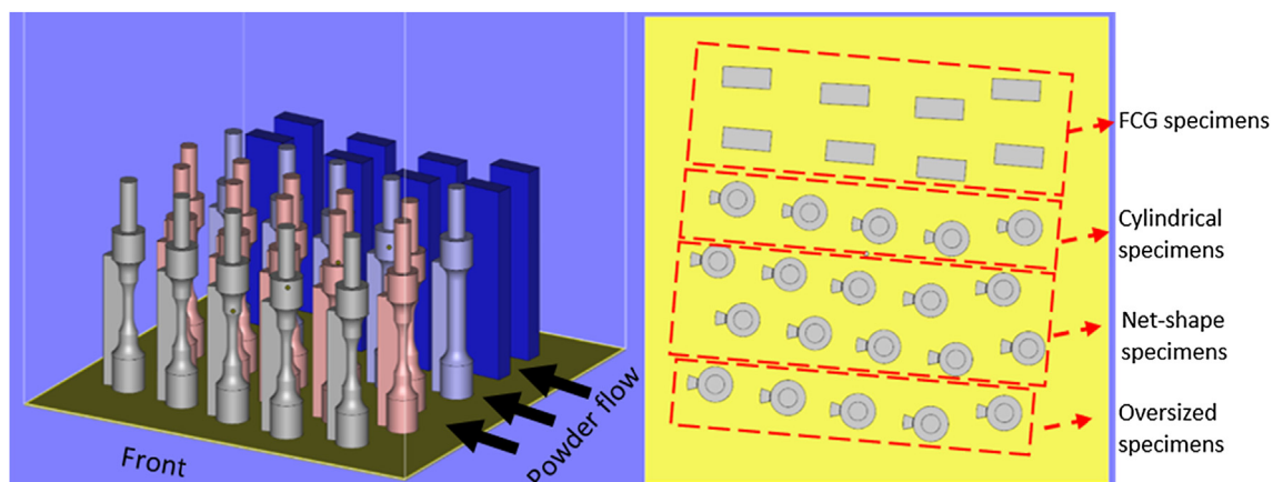
Fig. 2. LB-PBF build layout, showing net-shape (NS), oversized, and cylindrical specimens for fatigue testing as well as parallelepiped specimens for FCG testing.
