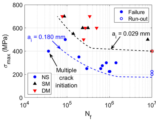
Fig. 13. Comparison of experimental stress-life fatigue data and the conservative fatigue curve predicted based on the most severe defect expected in the material. FCG simulations were performed using NASGRO.
