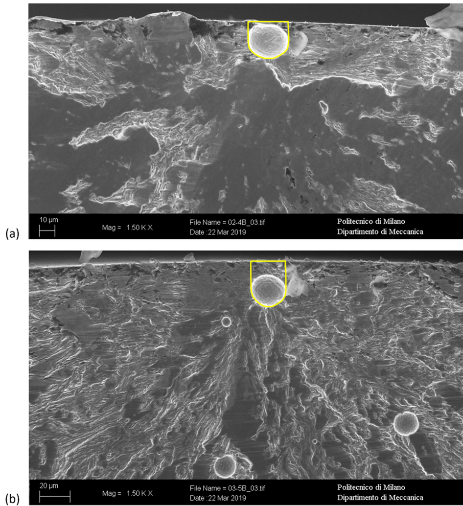
Fig. 11. Examples of typical fracture surfaces for the machined conditions: (a) a SM specimen fractured after 2.33 \times 10^5 cycles subjected to a stress amplitude of 600 MPa; and (b) a DM specimen fractured after 3.42 \times 10^5 cycles subjected to a stress amplitude of 700 MPa.
