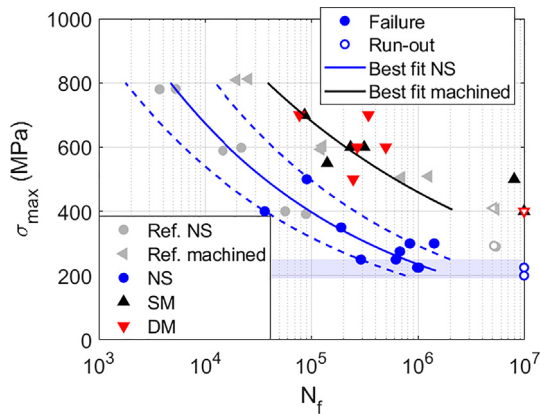
Fig. 9. Stress-life fatigue data representing the effect of machining allowance on the fatigue performance of LB-PBF 17-4 PH SS and their comparison with data adopted from [34]. The dotted blue lines represent the 95% scatter band of the experimental data for NS specimens. (For interpretation of the references to colour in this figure legend, the reader is referred to the web version of this article.)
