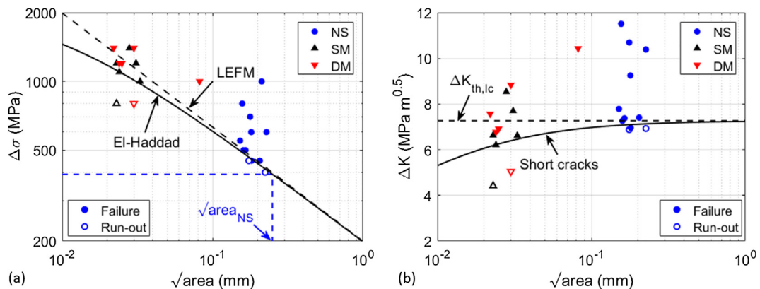
Fig. 12. Kitagawa diagram in terms of (a) stress, and (b) SIF range.
